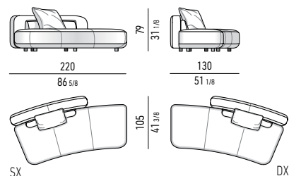
ELEMENTO PENISOLA CM 220 OPEN-END ELEMENT CM 220
