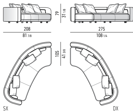
ELEMENTO TERMINALE CM 208 ELEMENT WITH 1 ARMREST CM 208
