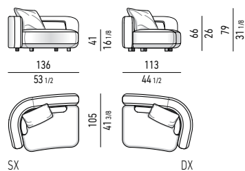
ELEMENTO TERMINALE CM 136 ELEMENT WITH 1 ARMREST CM 136
